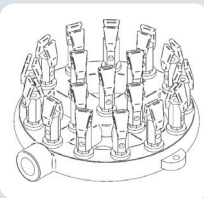
DUCK-TIP BURNER
